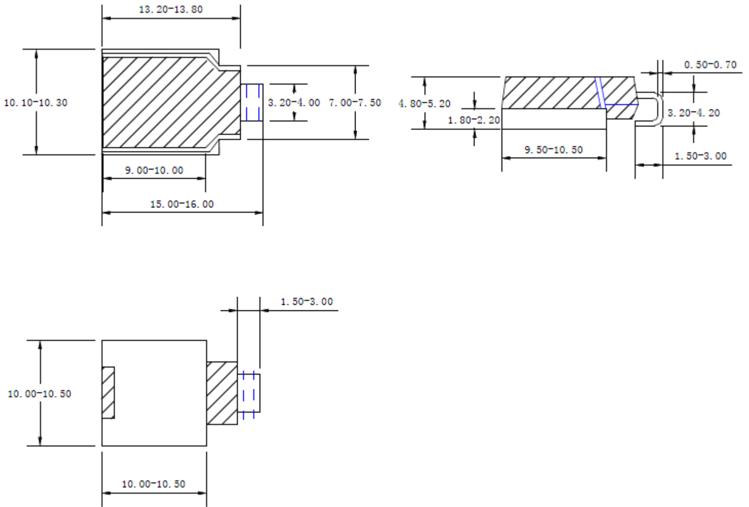
DO-218AB/SMD-BLOCK (mm)
